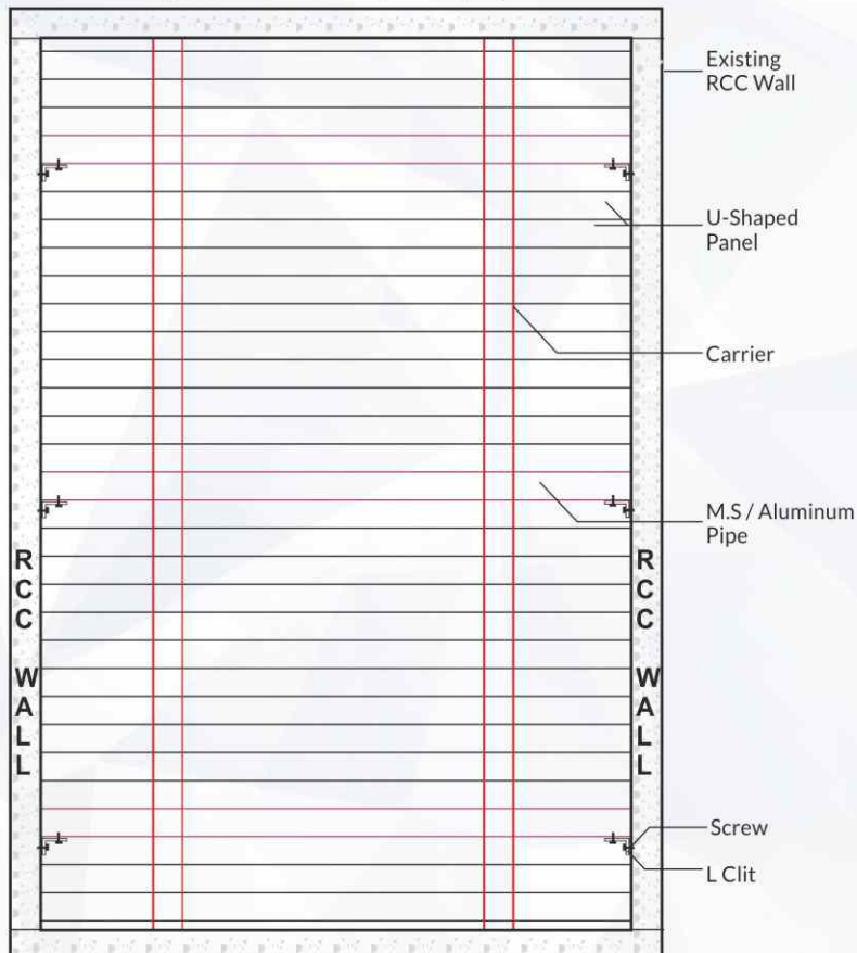
U - Shaped Box Louver (Baffle) Systems.
